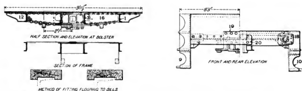
Figs. 3652-3656. Sections Through Underframe of Steel Tender for Atlantic (1—4—2) Locomotive. P. R. R.
